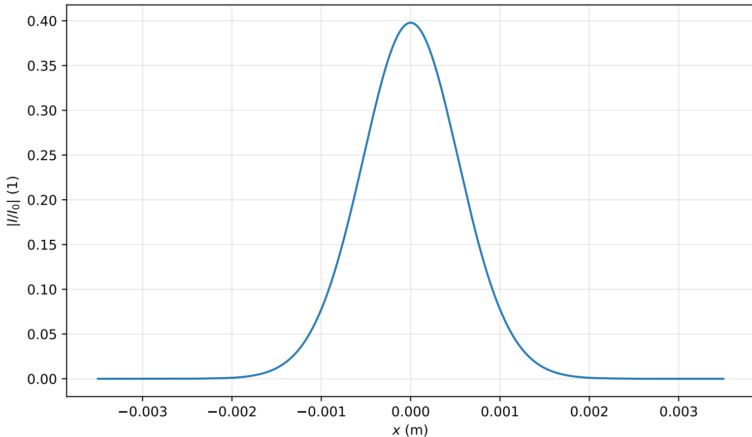
Intensity profile I(x, y = 0, z = 2.866m)/I_0 , P_{in}=0.2P_{cr} , artificial time
